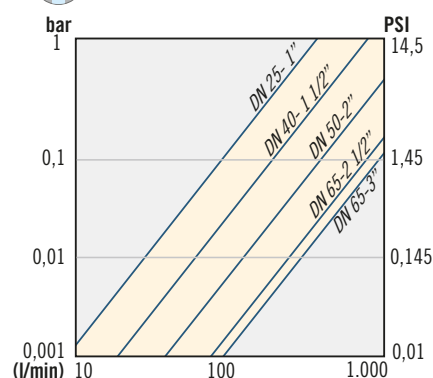
MODELO "T" / "T" MODEL
